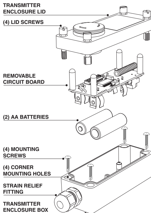
IMAGE 4: TRANSMITTER ASSEMBLY
